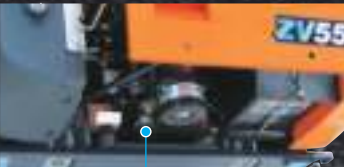
Automatic V-Belt Tensioner
