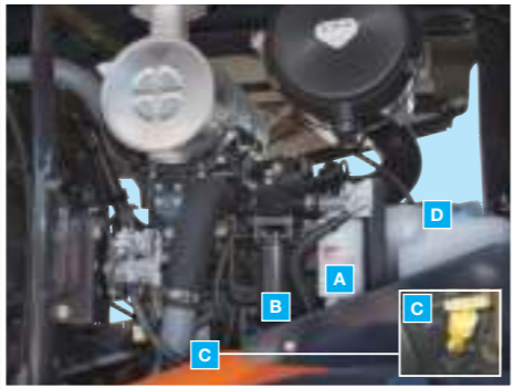
A Fuel pre-filter B Main fuel filter C Engine oil gauge D Window washer tank
